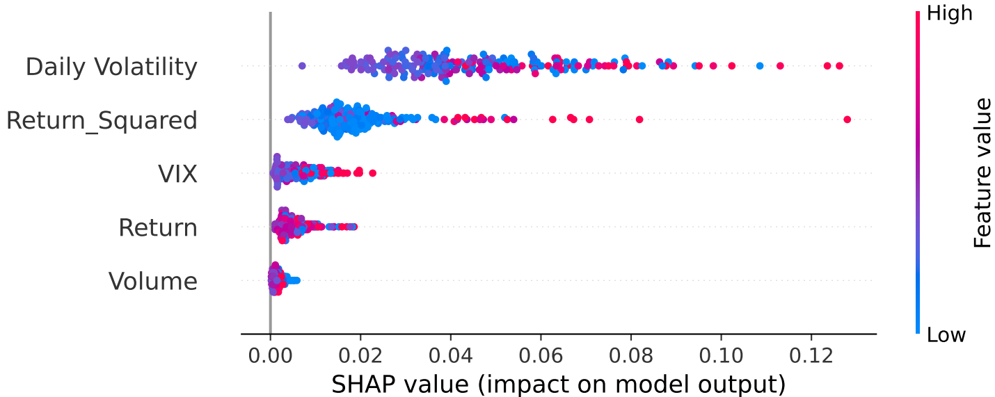
LSTM (VIX) — SHAP Beeswarm Plot
